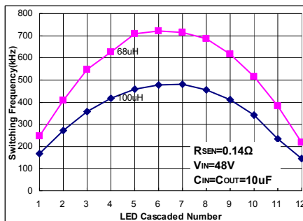
I_{OUT}=700mA
