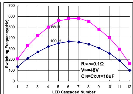
I_{OUT}=1000mA
